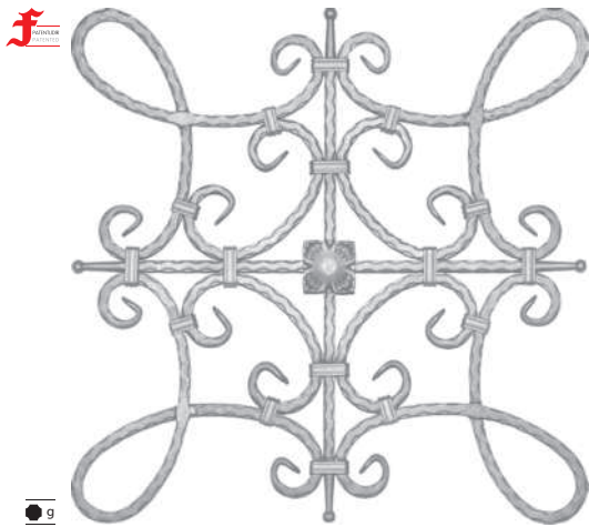
121212 AxBxH : 81.5x59.5x59.5 cm. 7,820 kg. ■ 12 mm.
